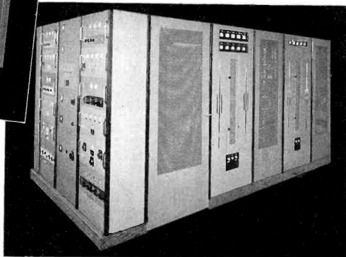
The first F-M relay transmitter (250 watts at 156 Mc) in the World, installed by R.E.L. for the Yankee Network in Boston, Mass., relaying to Paxton, Mass. (45 miles, airline) and in operation 16 hours daily since May, 1939.
